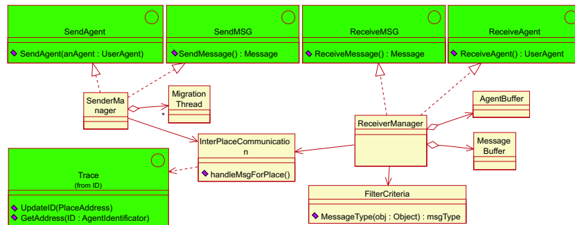
Fig. 4. SendReceive Component
