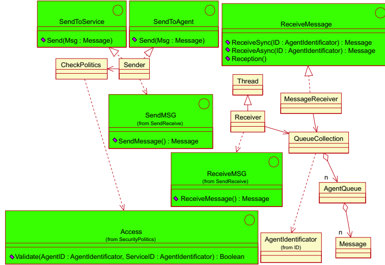
Fig. 6. Communication Component
