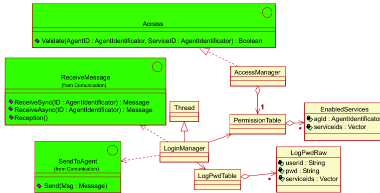
Fig. 7. SecurityPolitics Component
