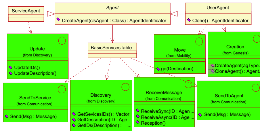
Fig. 8. Agent Component
