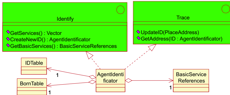
Fig. 3. ID Component
