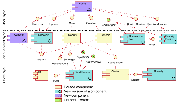
Fig. 11. Components overview in the industrial domain
